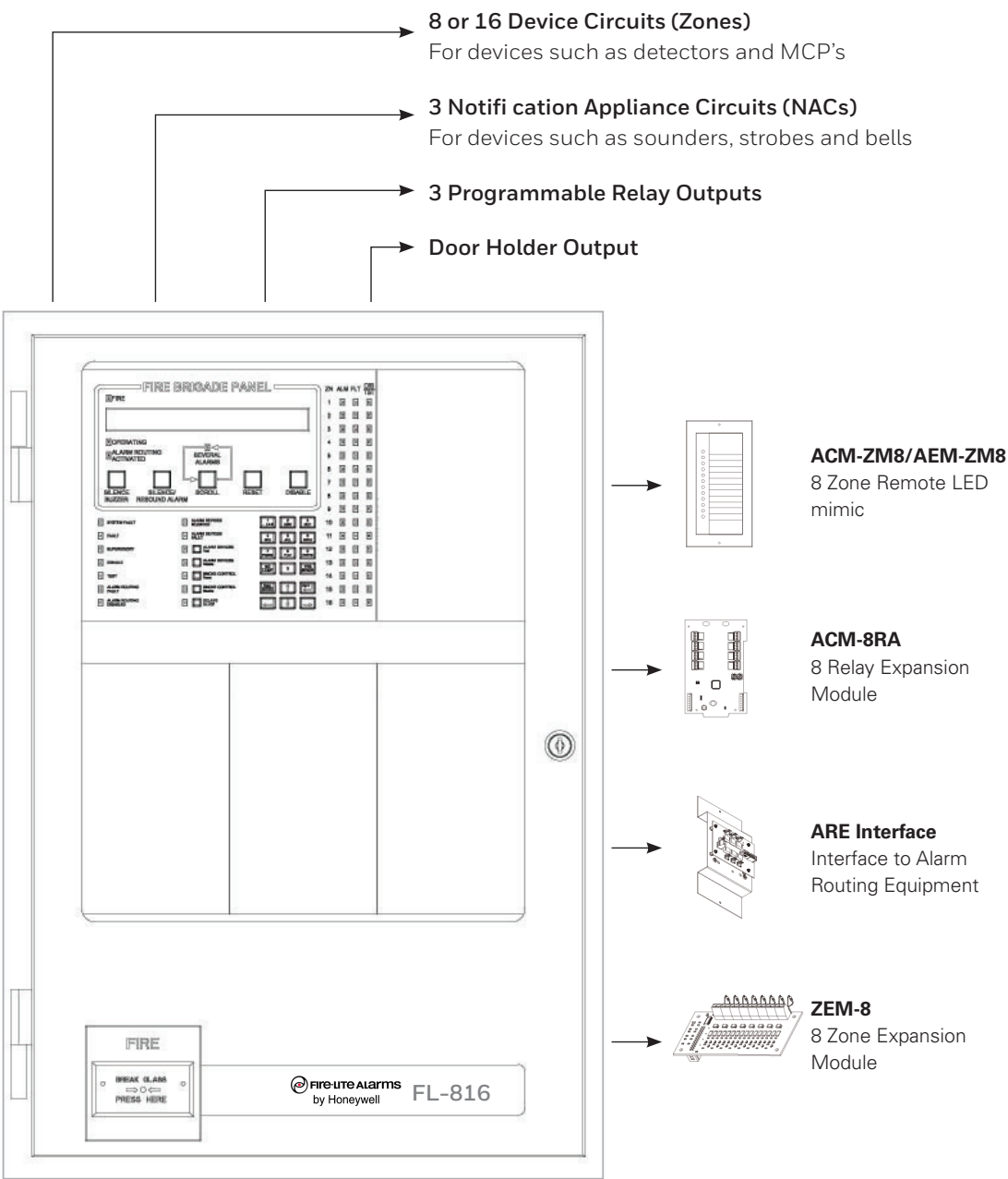
FL-816 Connection Overview
